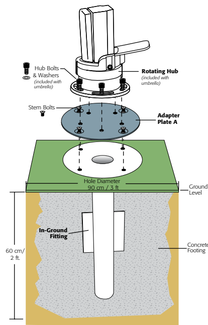
IN-GROUND INSTALL
