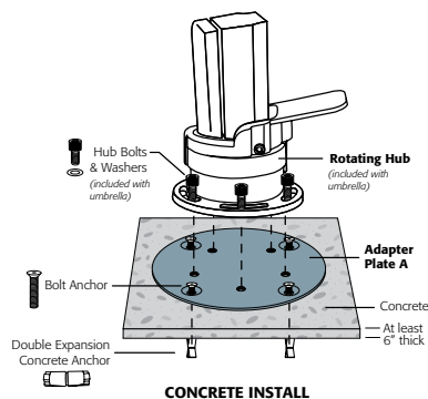
CONCRETE INSTALL
